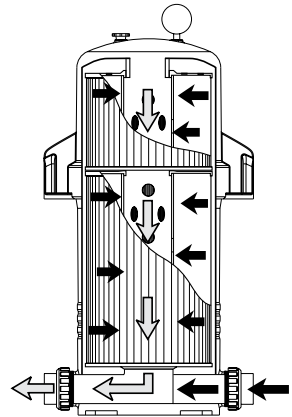
FLOW DIAGRAM
